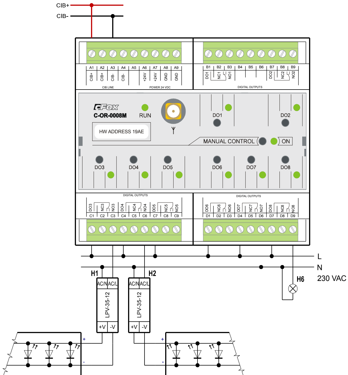
Fig. 6.1.1.1 Example of switching power supplies for LED by C-OR-0008M module.
