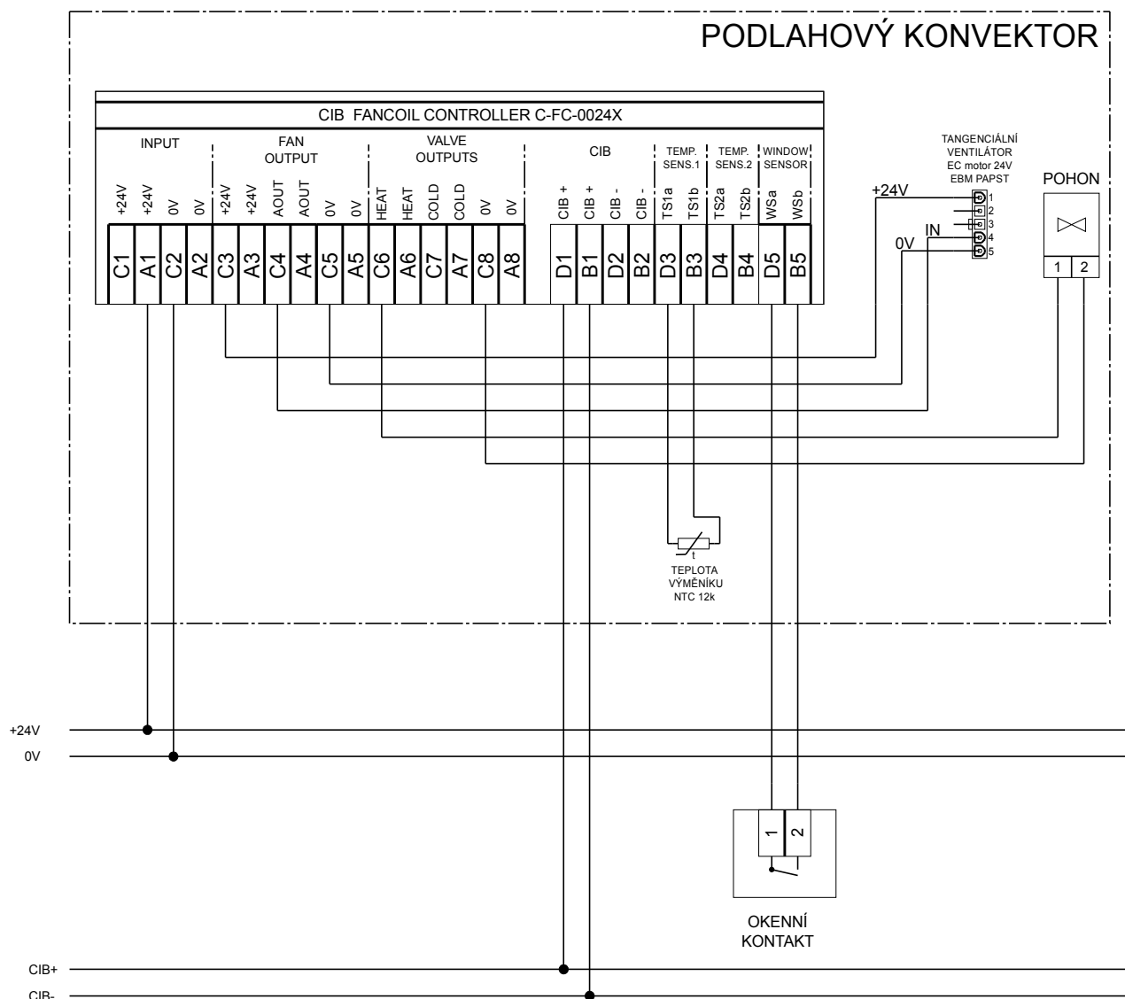
Fig. 4.4.1.1 Example of two-pipe convector by ISAN with EC motor by EBM Papst
