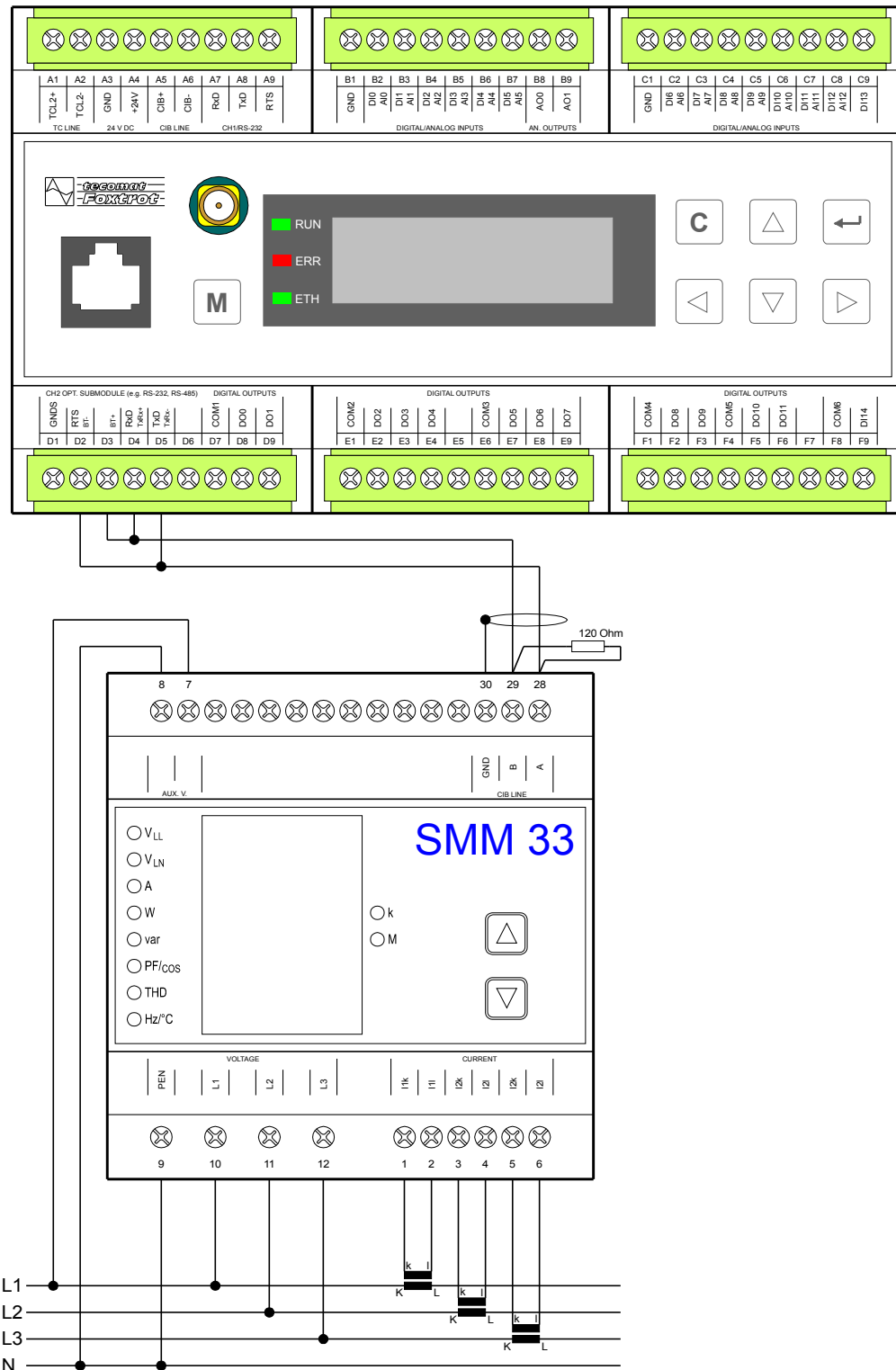
Fig. 11.5.1 Example of connection of SMM 33 - analyzer of 3phase power network.
